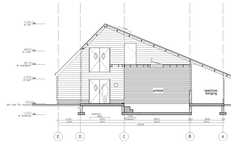
Doorsnede BB - binnengevel as 5
